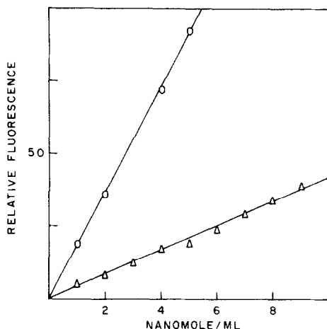
Fig. 2 Fluorescence of 5-(2-carboxyphenyl)-5-hydroxy-1-methyl-3-phenyl-2-pyrrolin-4-one (II, R = CH 3 ) (- o -) and the fluorescence generated from sarcosine (- Δ -).
